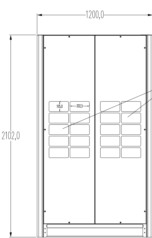
Air Entry
